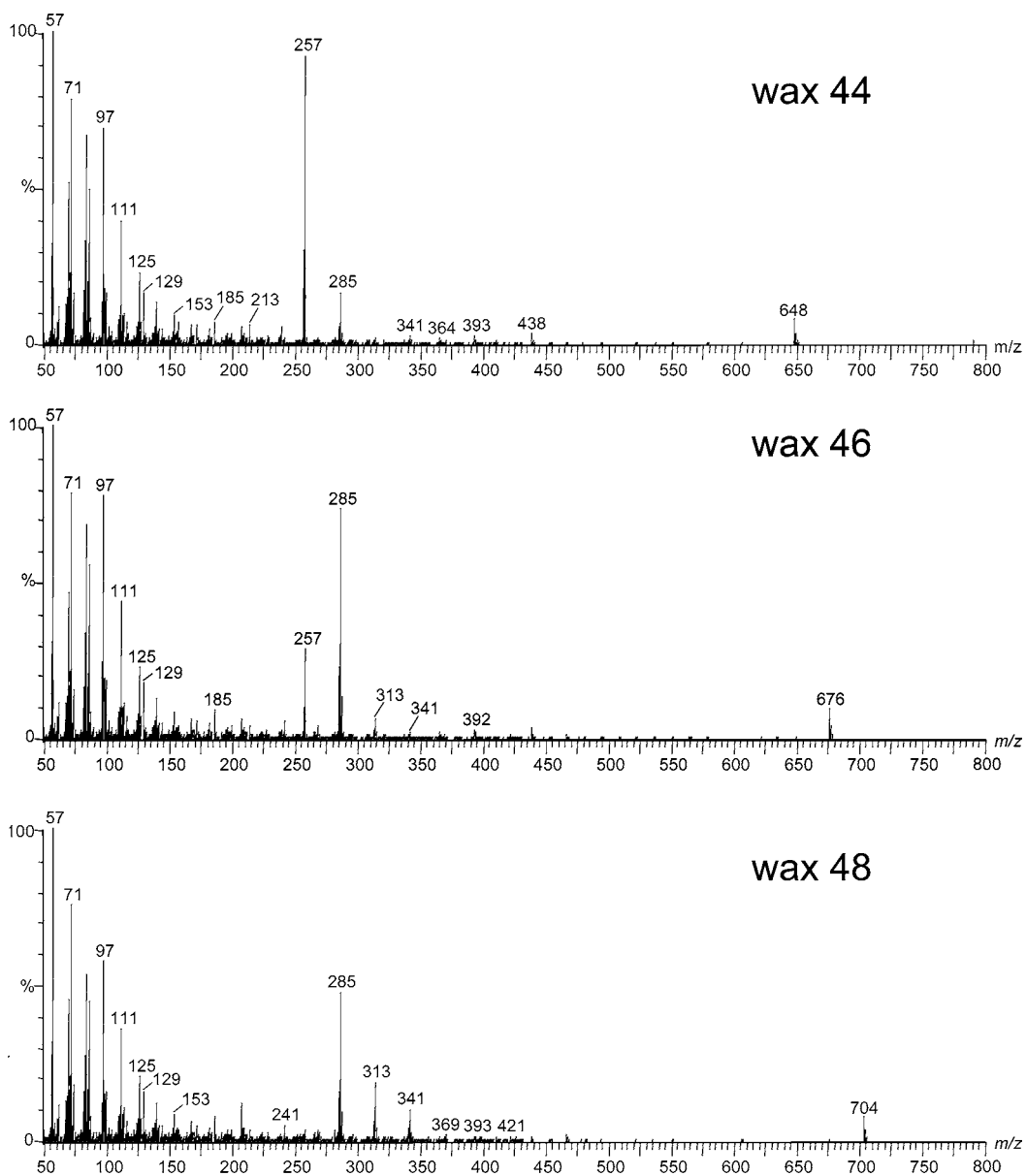
Figure 3. Mass spectra of the chromatographic peaks corresponding to (a) wax C 44 , (b) wax C 46 , and (c) wax C 48 . (The lengths of the waxes have now been correctly identified.)
